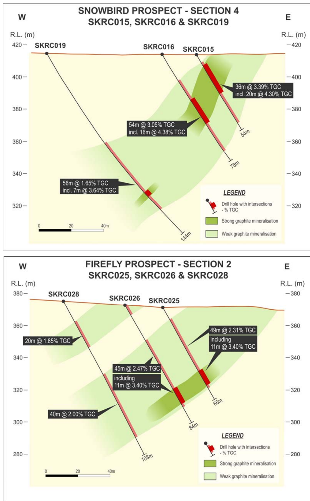
Figure 3: Cross-section, Snowbird and Firefly Prospects
