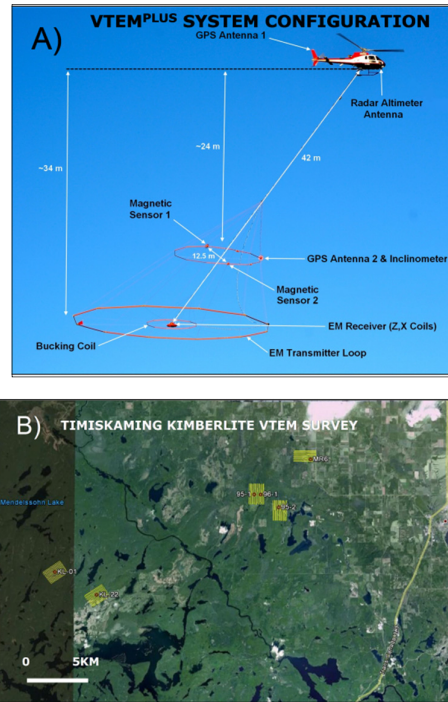
Figure 1: A) VTEM Plus helicopter EM system configuration with horizontal magnetic-gradiometer; B) Timiskaming Kimberlite VTEM survey locations, showing flight lines and kimberlites (red circles)
