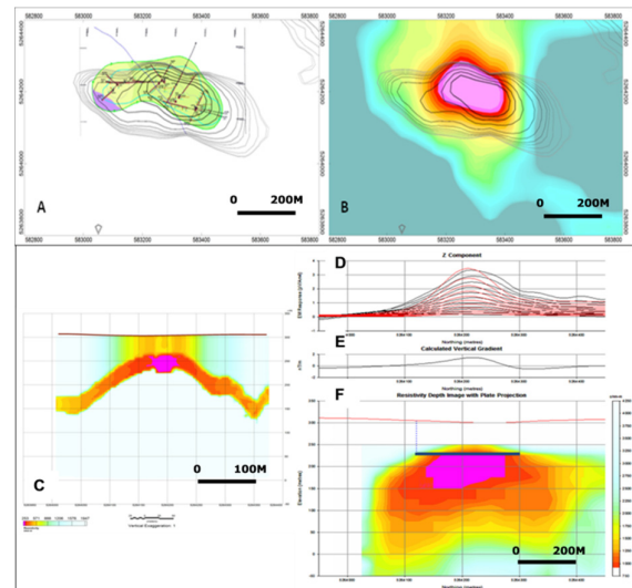
Figure 2: A) Geological Outline of kimberlite pipe 95-2 in plan view with CVG contours and B) grid of TEM early time gate (ch8 = 39-45 \mu sec dB/dT) with CVG contours (B) (CVG-calculated vertical gradient of magnetic field)); C) Laterally Constrained Inversion; D) dB/dt Z measured response in black and forward model response in red; E) Calculated vertical gradient of total magnetic intensity; and F) plate model and RDI section, all along the anomaly on north-south Line 1050.
