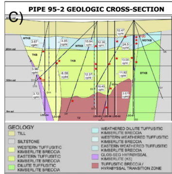
Figure 1: C) Geologic cross-section across 95-2 kimberlite (courtesy Stornoway Diamond Corporation).
